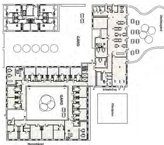
Markplan
